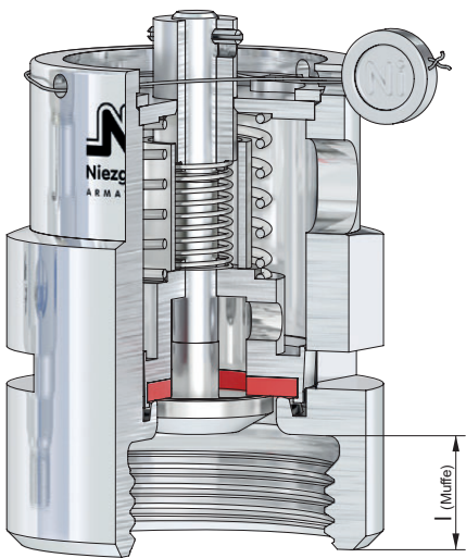
G1 - Muffe
